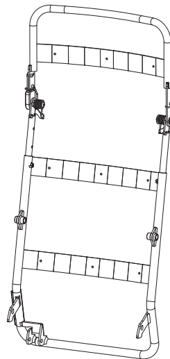
Backrest RG70 - Step Joint (30° KS) - AR Mount. 175mm Art-No. RG 70-015692
