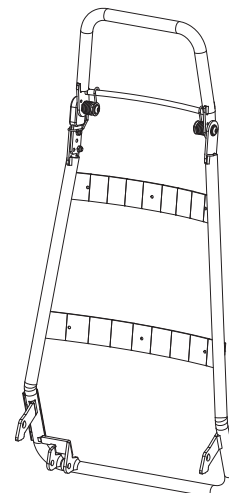
Backrest RG60 conical - Step Joint (30° KS) - Without AL Mounting Art-No. RG 60-001045
